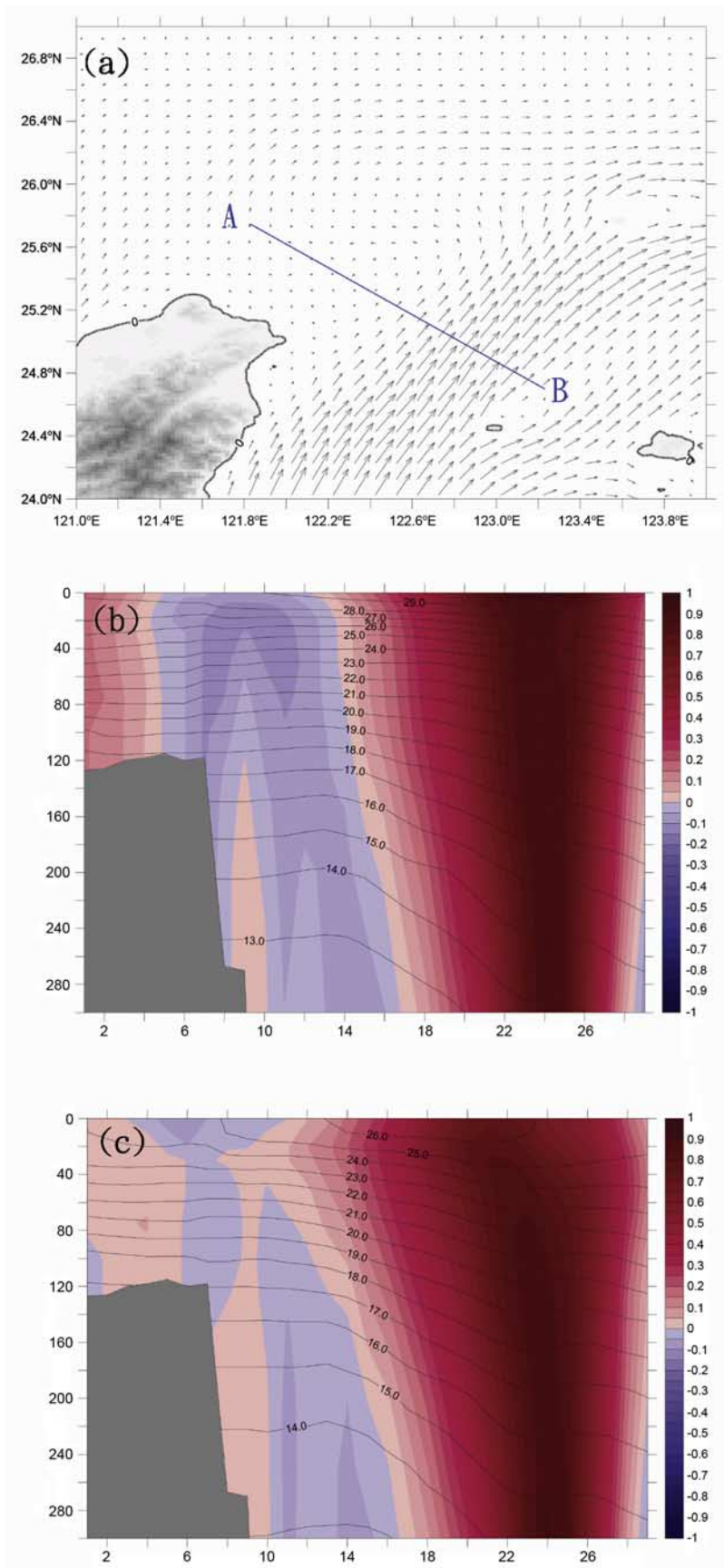
Figure 8. (a) The blue segment AB across the Kuroshio indicates the position of the transection. Vertical section of along-stream velocity together with temperature contours in (b) summer and (c) winter.
