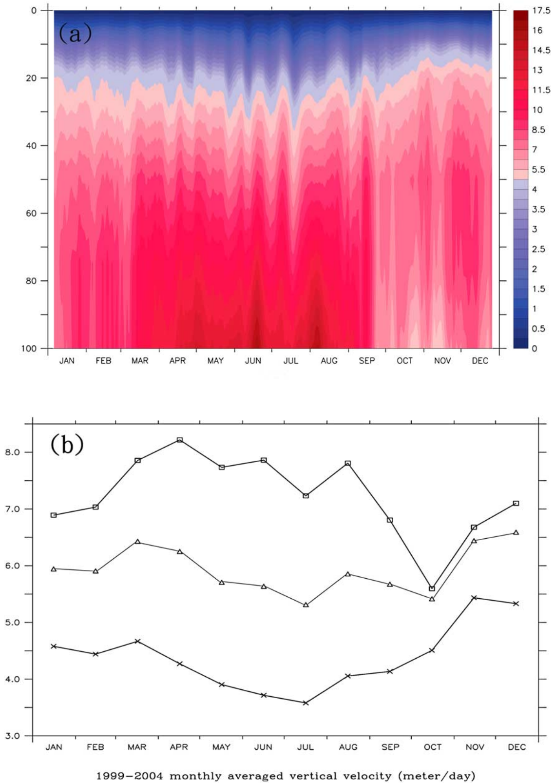
Figure 9. (a) Seasonal variation of the vertical velocity in the upper 100 m based on the model’s 10-day running averaged values from 1999 to 2004. (b) Monthly averaged vertical velocity in the upper 100 m (open square), in the top 30 m (cross), and in the upper 60 m (open triangle).
