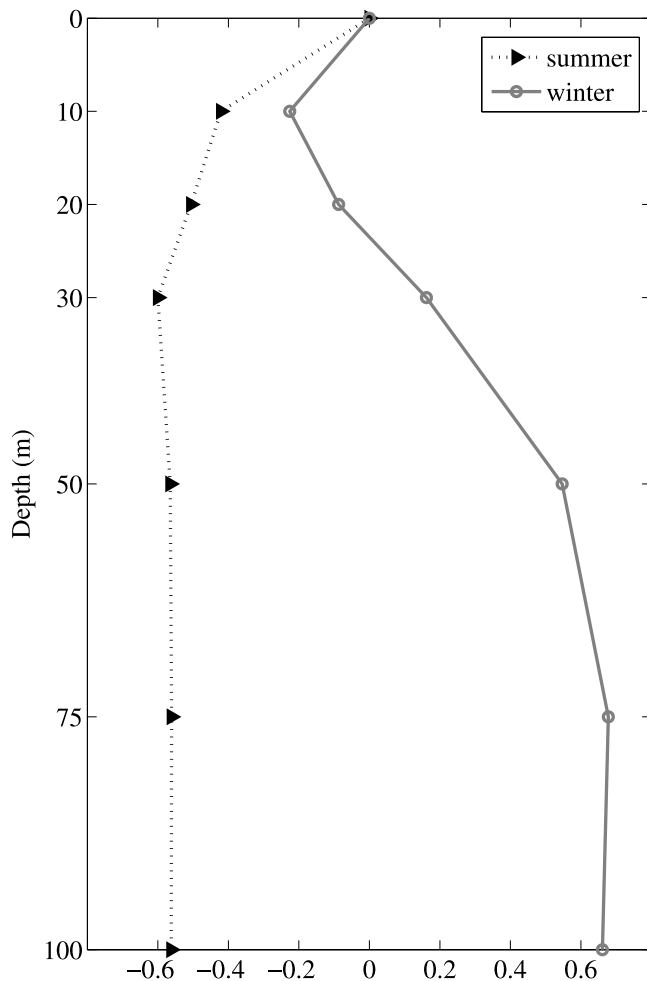
Figure 6. The vertical velocity w_{wind} in the upper 100 m in summer (dashed line) and in winter (solid line) in blue box of Figure 1b.
