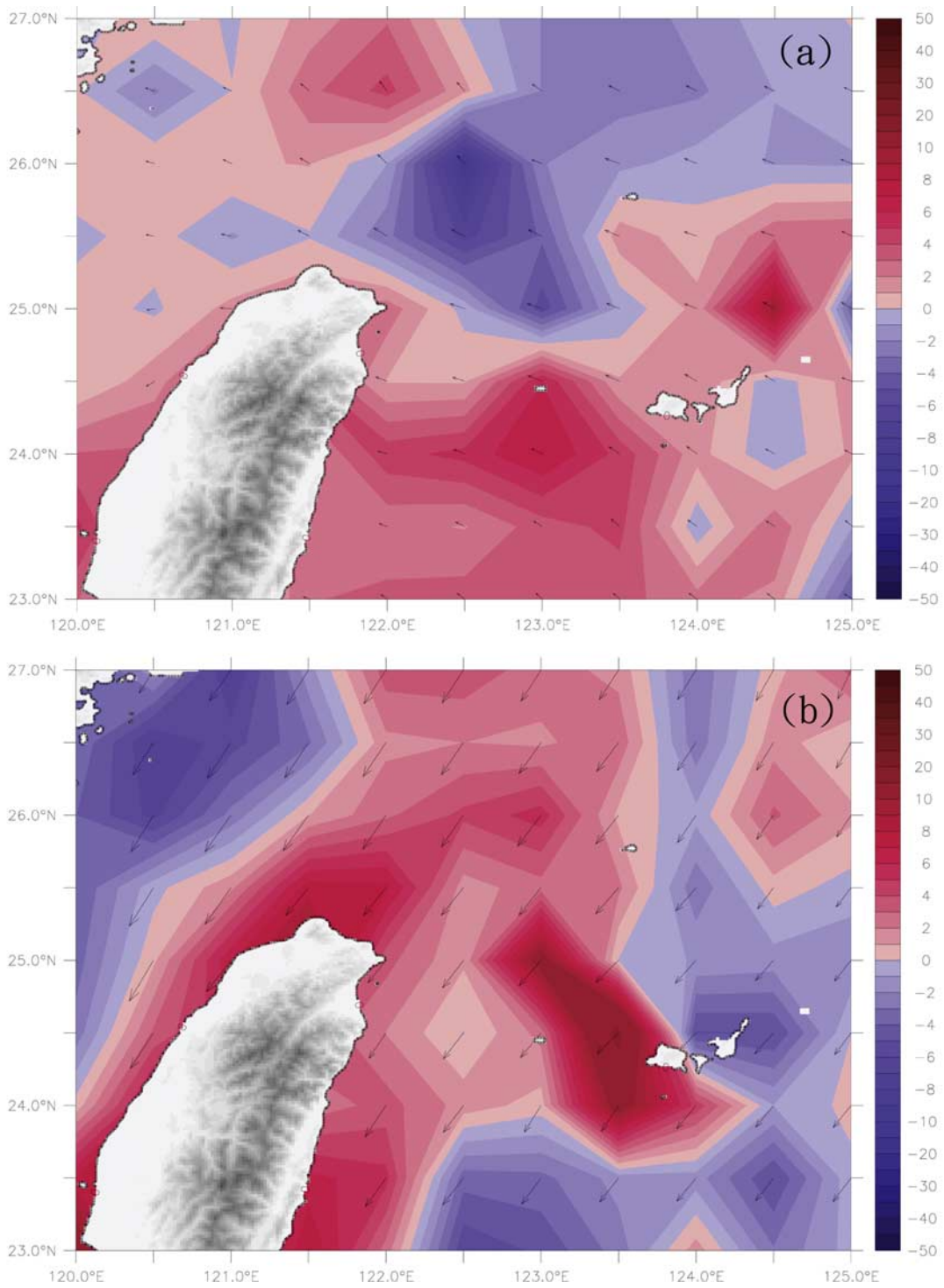
Figure 4. Averaged wind stress curl with wind field during the period from 1999 to 2004 in (a) summer and (b) winter.
