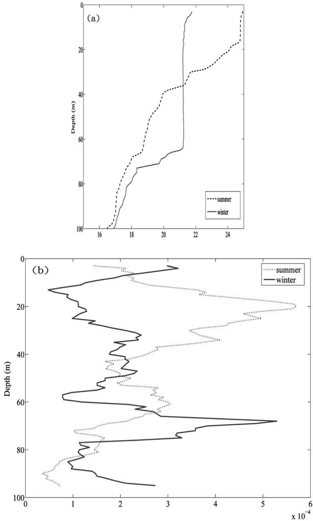
Figure 7. (a) CTD temperature profile in the upper 100 m in summer (dashed line; 122.25°E, 25.33°N) and in winter (solid line; 122.25°E, 25.42°N). (b) Buoyancy frequency squared at the upper 100 m in summer (dashed line) and in winter (solid line).
