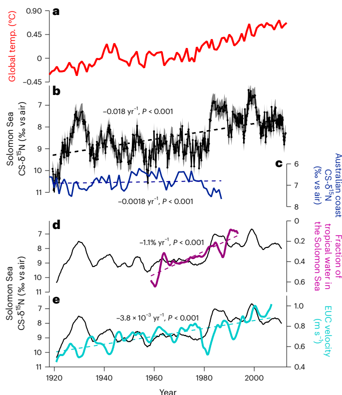
Fig. 2 | Long-term declines in the Solomon Sea coral skeletal nitrogen isotope ratios are associated with twenty-first century change in the climate and oceanic processes in the Pacific and globally. a , The rising trend of global surface temperature (temp.) 55 . b , The Solomon Sea CS- \delta^{15}\text{N} , with grey shadings representing the average 1\sigma of replicated samples. c , The published CS- \delta^{15}\text{N} record from the Australian coast is relatively constant over this period 29 . d , Radiocarbon-based calculations of the fraction of eastern equatorial water in the upper Solomon Sea indicate a decline in tropical water in the Solomon Sea 38 . e , The EUC is shown to intensify over the last century (maximum EUC strength and zonal velocity at 0° N, 146° W and 112 m depth) 44 . Note that all the data series in d and e have been smoothed by a 3-year running mean.
