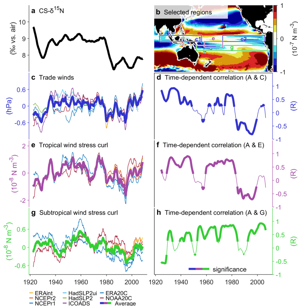
Extended Data Fig. 6 | Correlation between CS- \delta^{15}\text{N} and tropical vs. subtropical winds. a , 7-year running mean of the Solomon Sea CS- \delta^{15}\text{N} . b , Wind stress curl difference (color, in 10^{-7} \text{ N m}^{-3} ) between 1960–1980 (negative PDO phase) and 1980–2000 (positive PDO phase). Boxes indicate regions where tropical and subtropical winds are computed from data reanalysis product 58,68–73 . The strength of the equatorial trade winds in c is computed from a large-scale tropical SLP gradient ( \Delta\text{SLP} ) between the central/east Pacific ( 160^\circ\text{W} – 80^\circ\text{W} ) and the west Pacific/Indian Ocean ( 80^\circ\text{E} – 160^\circ\text{E} ) (box c2 and c1). The index is computed with SLP anomalies from monthly climatology and averaged over grid cells within 5^\circ latitude of the equator, then averaged with 7 years window. The tropical and subtropical wind stress curl anomalies in panel e and g are computed from monthly climatology and averaged over the area in box e ( 5^\circ\text{S} – 15^\circ\text{S} ,
