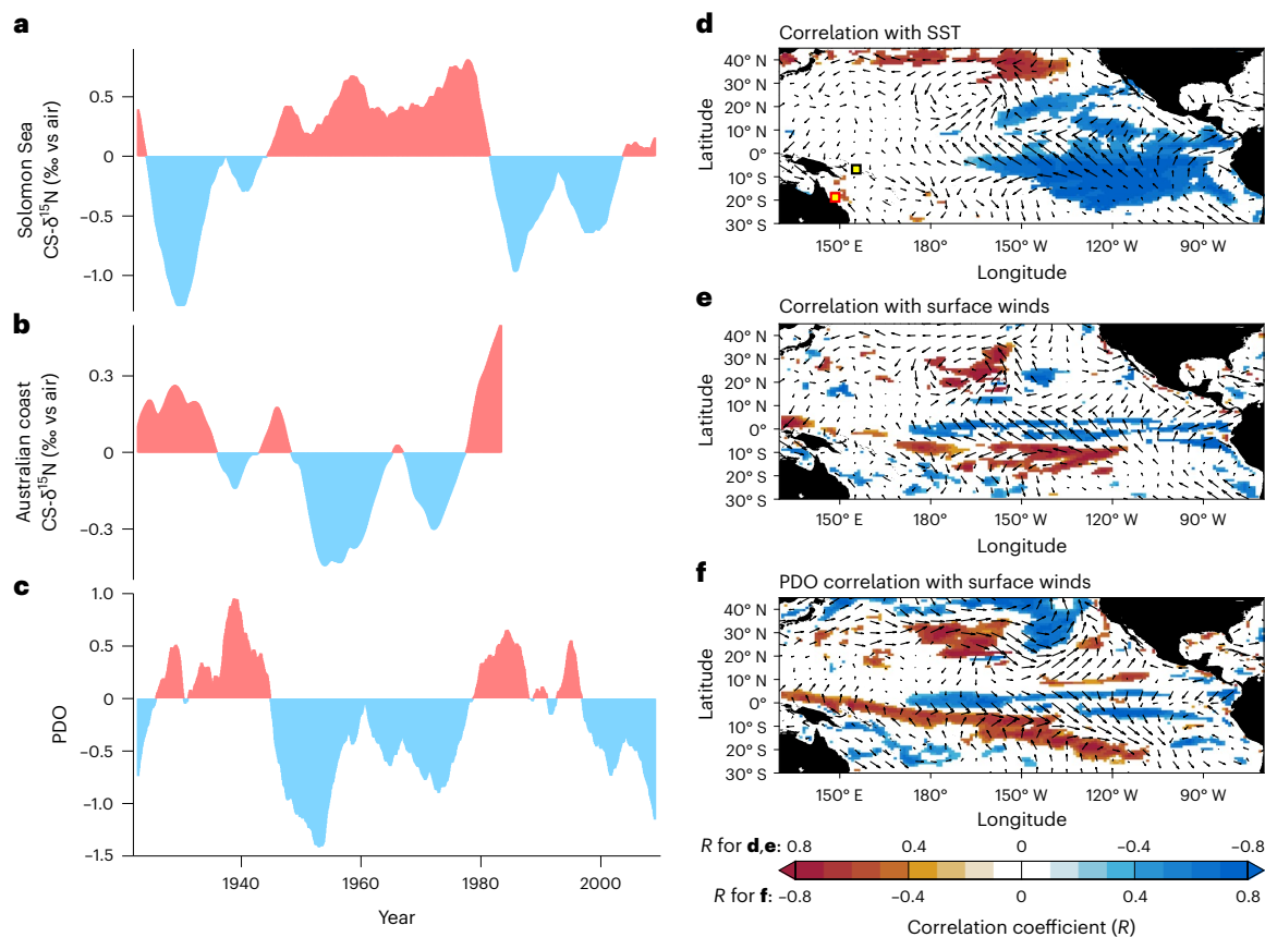
Fig. 3 | Decadal changes in the coral skeletal nitrogen isotope ratios are linked to Pacific Decadal Oscillation. a–c, The decadal changes in the Solomon Sea CS- \delta^{15}\text{N} (a) are significantly correlated with the Australian coast CS- \delta^{15}\text{N} (ref. 29) ( r = -0.77 , P = 0.01 , 7-year running average; Methods) (b) and the PDO 56 ( r = -0.69 , P = 0.03 , 10-year running average, with PDO leading by 46 months; Methods) (c). In a–c, positive and negative anomalies from the mean values are indicated with red and blue, respectively. d, Changes in the Solomon Sea CS- \delta^{15}\text{N} are strongly correlated with basin-wide changes in the SST, especially with surface warming in the North Pacific, and surface cooling in the southeast Pacific. The locations of the Solomon Sea and Australian coast coral cores are shown in black and red squares. e,f, The Solomon Sea CS- \delta^{15}\text{N} is also strongly correlated with the Pacific surface wind field (e) that is similar to the PDO-like wind patterns (f). On both e and f, vectors show correlation coefficient with wind
